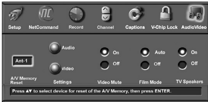
Figure 22. Audio/Video Menu
